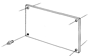
38 —Drilled, with Drive Rivet Fasteners
