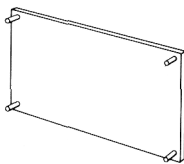
39 —Welded Stud Mounting (On Back of Panel)
